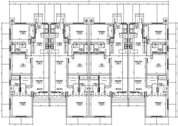
1 GROUND FLOOR PLAN
